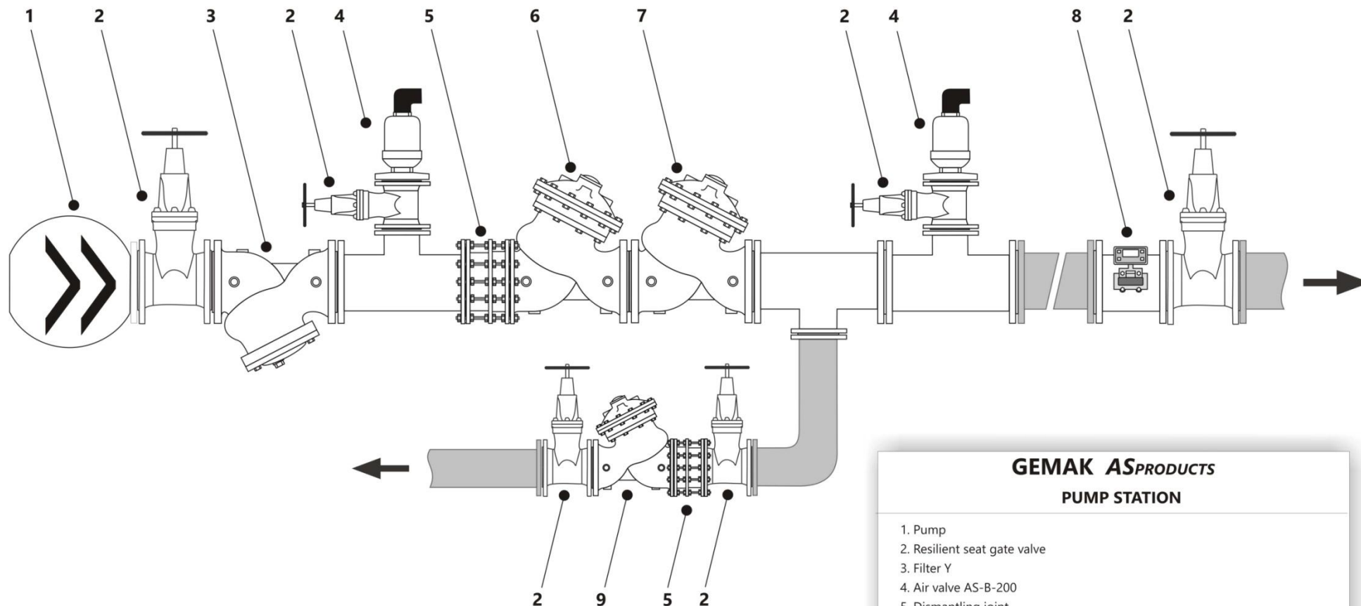
PUMP STATION TYPICAL INSTALLATION
